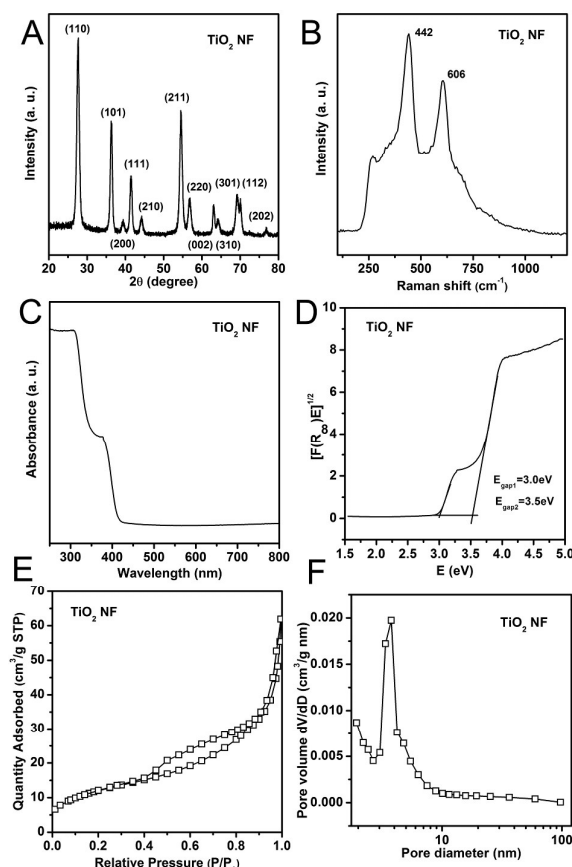
Fig. 2 (A) XRD pattern of the rutile \text{TiO}_2 nano-flower structure; (B) Raman spectrum of rutile \text{TiO}_2 nano-flower structure; (C) UV-Vis diffuse reflectance spectrum of rutile \text{TiO}_2 nano-flower structure; (D) Transformed UV-Vis diffuse reflectance spectrum of rutile \text{TiO}_2 nano-flower structure; (E) The \text{N}_2 adsorption-desorption isotherm of rutile \text{TiO}_2 nano-flower structure; (F) The pore size distributions of rutile \text{TiO}_2 nano-flower structure.
