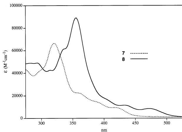
Fig. 1. UV–visible spectra of 7 and 8 ( \text{CH}_2\text{Cl}_2 , ambient temperature).
