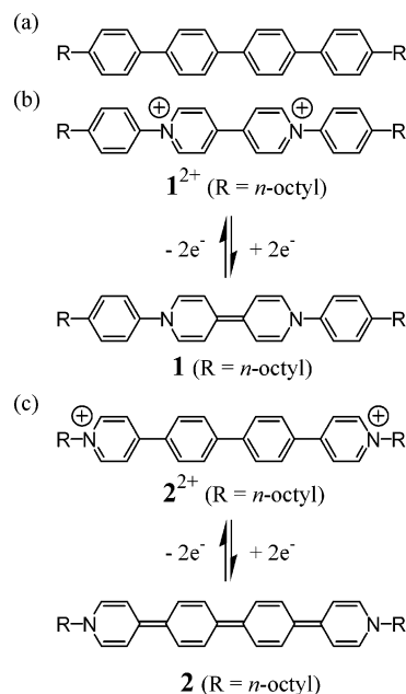
Figure 1. (a) p -Quaterphenyl (R = H), 4,4′′′-di- n -octyl- p -quaterphenyl (R = n -octyl); (b) phenyl viologen (R = H), 1,1′-bis(4- n -octylphenyl)-4,4′-bipyridinium (R = n -octyl); (c) extended viologen 2 and its dication 2^{2+} .
