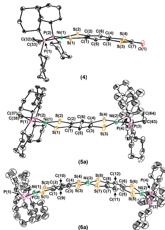
Figure 1. Thermal ellipsoid plots of [(dcpe)Ni(S 2 C 6 H 2 S 2 C=O)] ( 4 ; 50%), [(dcpe)Ni] 2 (S 2 C 6 H 2 S 2 ) ( 5a ; 50%), and [(dcpe)Ni(S 2 C 6 H 2 S 2 )] 2 Ni ( 6a ; 40%). H atoms are omitted for clarity.
