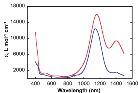
Figure 4. UV–vis and near-IR spectra in an N,N -dimethylformamide solution of [(\text{dcpe})\text{Ni}(\text{S}_2\text{C}_6\text{H}_2\text{S}_2)\text{M}(\text{S}_2\text{C}_6\text{H}_2\text{S}_2)\text{Ni}(\text{dcpe})] ( \text{M} = \text{Ni} , red; \text{M} = \text{Pt} , blue).
