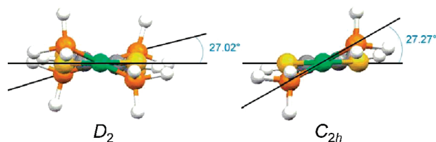
Figure 3. View of 5a' along the Ni–Ni axis in both the D_2 and C_{2h} point groups. For both geometries, the central \text{NiS}_4\text{Ni} unit is essentially planar. In D_2 , the two \text{P}_2\text{Ni} planes are staggered at 54.04^\circ relative to each other and at 27.02^\circ in opposite directions relative to the central \text{NiS}_4\text{Ni} plane. In C_{2h} , the two \text{P}_2\text{Ni} planes are coincident and form a dihedral angle of 27.27^\circ with the \text{NiS}_4\text{Ni} plane.
