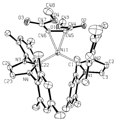
Figure 4. ORTEP diagram of 6 \cdot 3\text{C}_6\text{D}_6 . Hydrogen atoms and d_6 -benzene molecules are omitted for clarity. Thermal ellipsoids are drawn at the 50% probability level.
