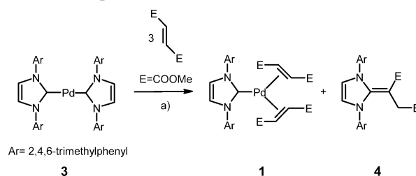
Scheme 2. Equilibrium Bis-NHC/Mono-NHC– \text{Pd}^0\text{–DMFU} a
