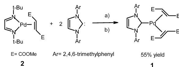
Scheme 3. Synthesis of \text{Pd}^0(\text{NHC})(\text{dmfu})_2 ( 1 ) a
