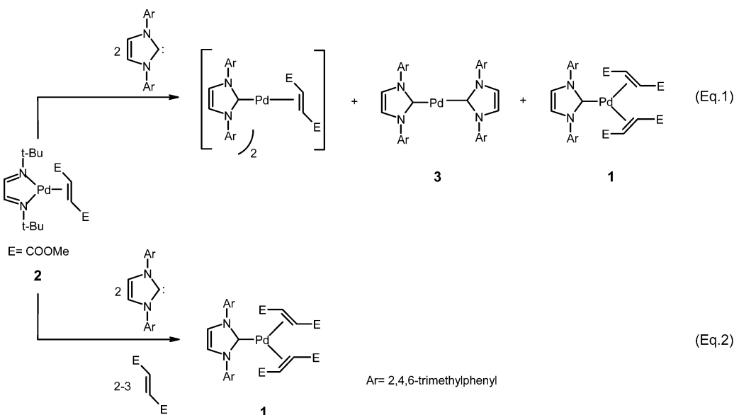
Scheme 2. Equilibrium Bis-NHC/Mono-NHC– \text{Pd}^0\text{–DMFU} a
