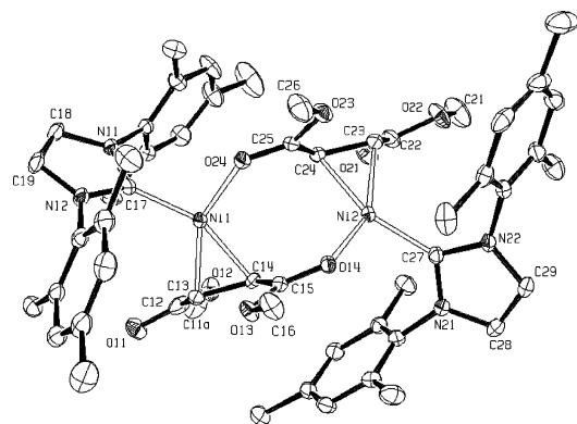
Figure 5. ORTEP diagram of 7·H 2 O. Hydrogen atoms, the water molecule, and disordered atoms are omitted for clarity. The methoxy group on C(12) is disordered over two positions in a 66:34 ratio. Thermal ellipsoids are drawn at the 30% probability level.
