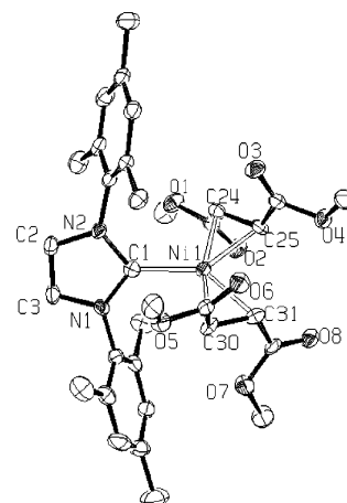
Figure 3. ORTEP diagram of 5 . Hydrogen atoms are omitted for clarity. Thermal ellipsoids are drawn at the 50% probability level.
