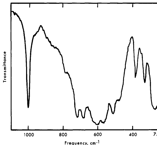
Figure 1. Infrared spectrum of solid chromium oxide trifluoride, \text{CrOF}_3 .
