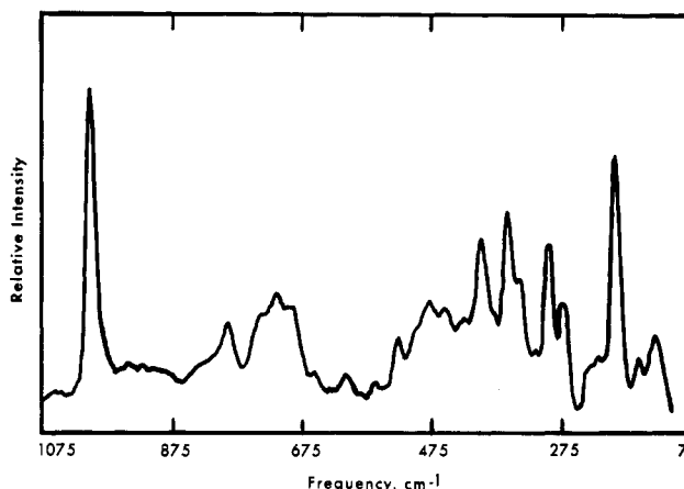
Figure 2. Raman spectrum of solid chromium oxide trifluoride, \text{CrOF}_3 .
