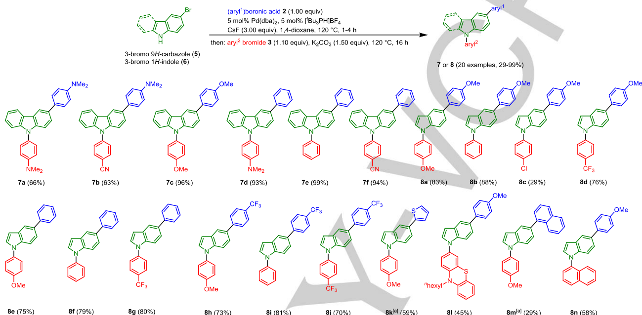
Scheme 2. Sequentially Pd-catalyzed arylation-amination consecutive three-component synthesis of 3,9-diaryl 9 H -carbazoles 7 and 1,5-diaryl 1 H -indoles 8 . ([ al ] aryl 1 -B(pin) was used.)
