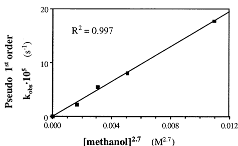
Fig. 2. Dependence of reaction 1 on the methanol concentration in \text{C}_6\text{D}_6 at 22°C. [\text{I}]_0 = 12.3 mM.
