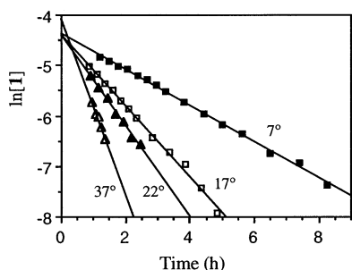
Fig. 1. First order plots for reaction 1. [\text{MeOH}] = 98.4 mM; [\text{I}]_0 = 12.3 mM.
