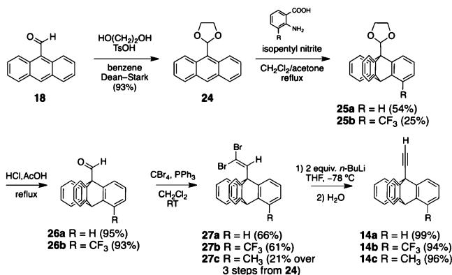
Scheme 3. Synthesis of Rotator/Axle Components 14a–c
