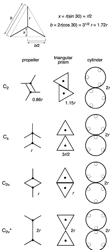
Figure 3. Geometrical analysis of two three-bladed rotators, approximated as propellers, triangular prisms, and cylinders, in C_2 , C_s , C_{2v} , and C_{2v}^* orientations. The distance from the axle to the blade is r , and the minimum distance between axes is given as a function of r .
