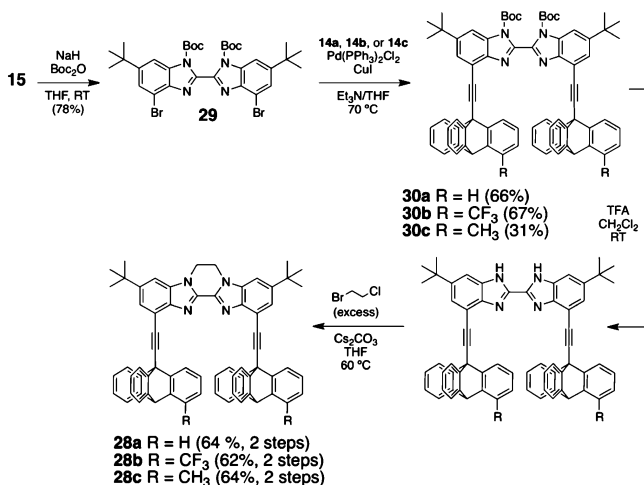
Scheme 4. Synthesis of Ethylene-Bridged Molecular Spur Gears 28a–c
