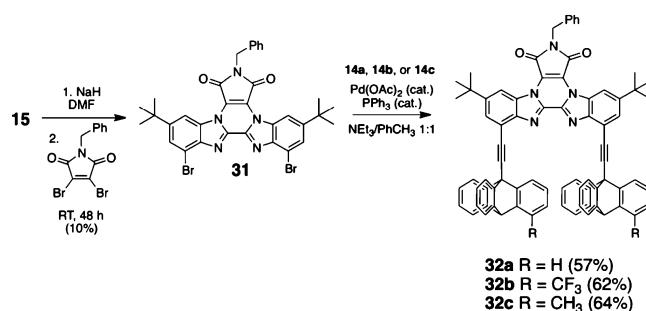
Scheme 5. Synthesis of Dioxypyrrole-Fused Spur Gears 32a–c
