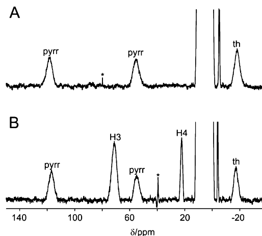
Figure 7. ^1\text{H} NMR spectrum of 7-Ni after the addition of (A) 0.25 equiv of pyridine- d_5 and (B) 0.25 equiv of pyridine (600 MHz, 200 K, \text{CD}_2\text{Cl}_2 ). Resonance assignments: pyr, pyrrole; th, thiophene; H3, H4, protons of coordinated pyridine.
