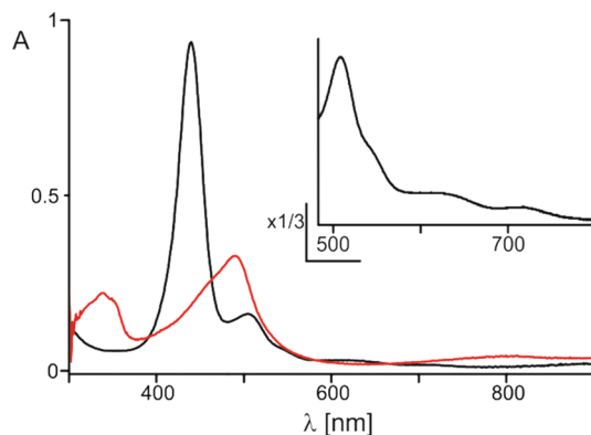
Figure 2. UV–vis absorption spectra (298 K, \text{CH}_2\text{Cl}_2 ) of 7 (black line) and [\mathbf{13}\text{-H}_2]^{2+} (red line). Inset: Q bands of 7 .
