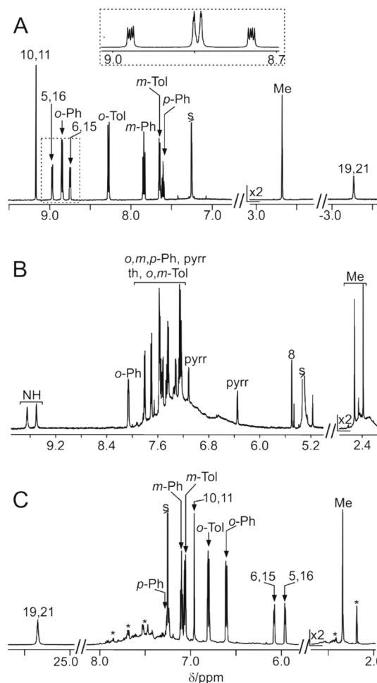
Figure 3. ^1\text{H} NMR spectra of (A) 7 ( \text{CDCl}_3 , 300 K), (B) \mathbf{12}'\text{-H}^+ ( \text{CD}_2\text{Cl}_2 , 300 K), and (C) [\mathbf{13}\text{-H}_2]^{2+} ( \text{CDCl}_3 , 300 K). Peak labels follow systematic position numbering or denote proton groups: o -, m -, p -Ph are the ortho, meta, and para positions of the meso -aryl groups. Inset: pyrrole region of 7 . Resonance assignments at trace B: pyr, pyrrole; th, thiophene. The broad resonance centered at 7.5 ppm in traces B and C is tentatively assigned to the unidentified products of oxidation.
