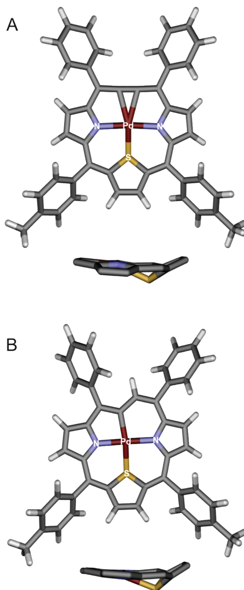
Figure 12. Geometries of 7 -Pd (A) and 14 -Pd (B) obtained in a DFT study. Projections emphasize the conformations of the macrocycles. Outer hydrogen atoms and meso substituents (bottom views) are omitted for clarity.
