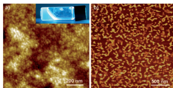
Figure 7. a) AFM height image of methylcyclohexane gel of 1a 3 ·CA. z scale = 10 nm. Inset shows a picture of the gel. b) AFM height image of 1a 3 ·CA spin-cast from a solution in MCH ( c=5.0\times 10^{-4} M). z scale = 6 nm.
