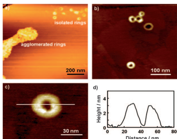
Figure 6. a–c) AFM height image of 1a 3 ·CA spin-coated from a solution in MCH ( c=2.0\times 10^{-4} M) and d) cross-sectional analysis along the white line in c). z scale = 6 nm in a) and 5 nm in b).
