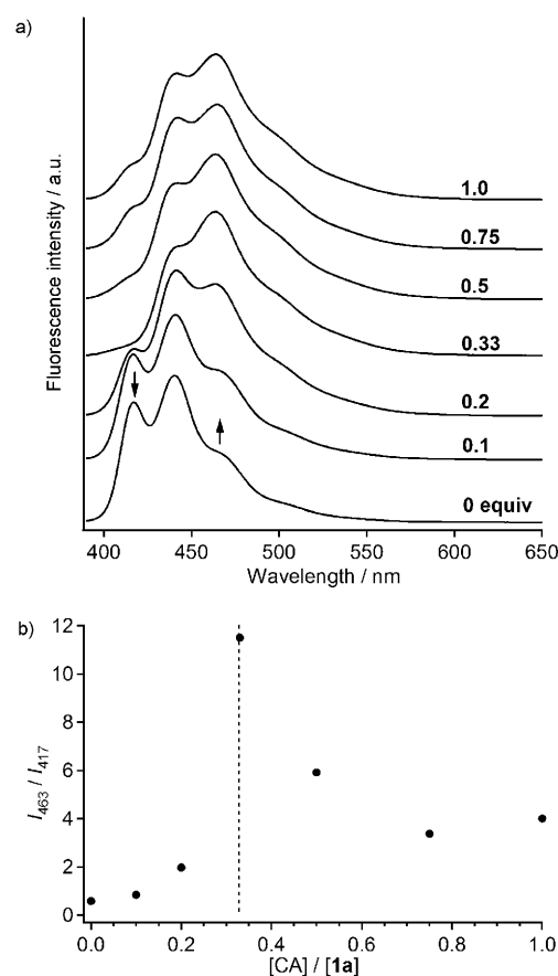
Figure 2. a) Fluorescence titration of 1a ( [\text{1a}] = 5 \times 10^{-4} M) with CA (0 to 1 equiv) in MCH; \lambda_{\text{ex}} = 349 nm. The spectra were normalized at their maxima. Arrows indicate the changes upon an increase in the concentration of CA. b) Plot of the ratio of fluorescence intensities at \lambda = 463 and 417 nm versus the [\text{CA}]/[\text{1a}] ratio. Dotted line indicates [\text{CA}]/[\text{1a}] = 0.33 .
