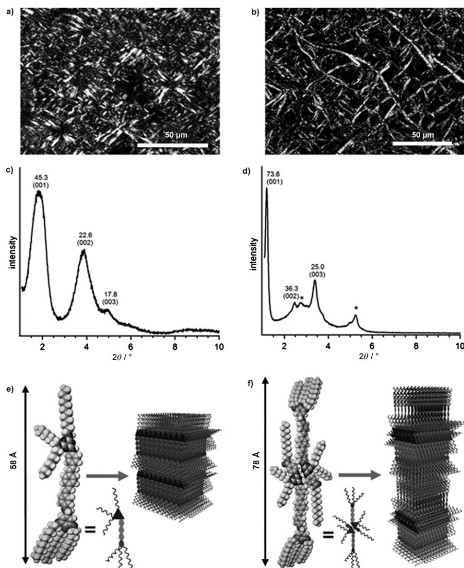
Figure 9. Polarized optical micrographs (a, b), XRD patterns (c, d), and proposed lamellar packing structures (e, f) of 1a (a, c, e) at 75°C and 1b (b, d, f) at 175°C upon cooling from the isotropic melt (cooling rate = 1°C min -1 ). The peaks designated by asterisk in d) are unidentified peaks.
