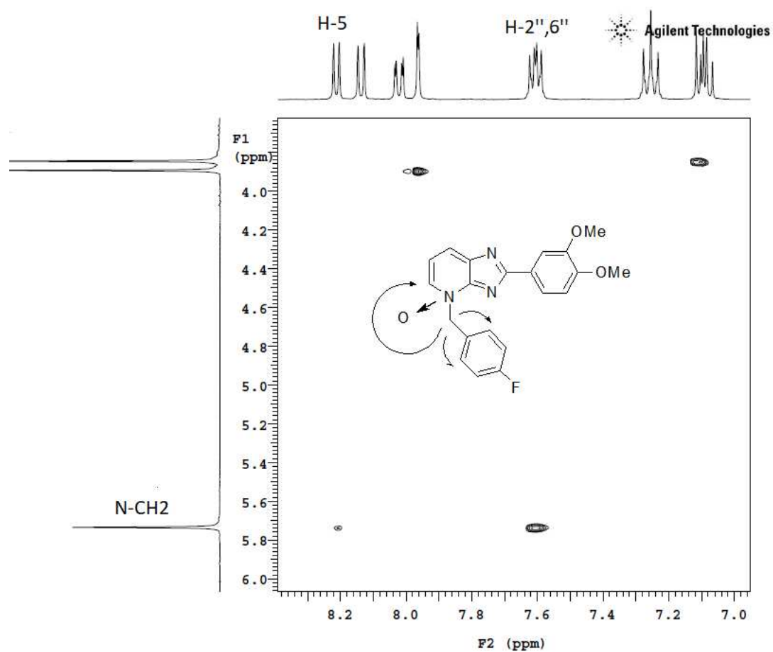
Fig 3. Partial NOESY spectrum of compound 7 showing cross peaks between N -CH 2 and H-5, 2'',6'' (in DMSO- d 6 ).
