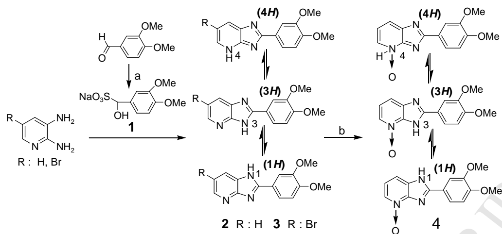
Scheme 1. Synthesis of 2 – 4 and their tautomeric forms.
