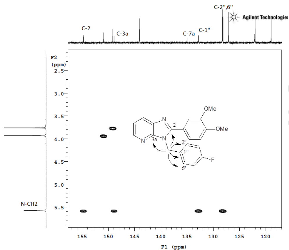
Fig. 4 gHMBC spectra of compound 6b , showing cross peaks between N\text{-CH}_2 / C-2, C-3a, C-1'', C-2'',6'' correlations (in \text{CDCl}_3 ).
