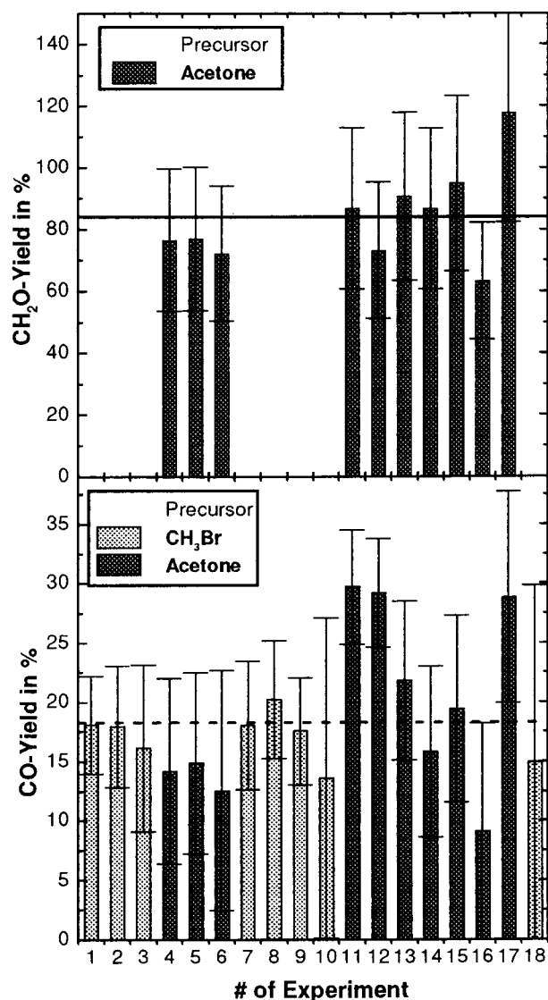
Figure 7. Plot of product yields for \text{CH}_2\text{O} and \text{CO} from reaction 1. Average values are marked by (—) and (---), respectively. The data are numbered according to Table 2.
