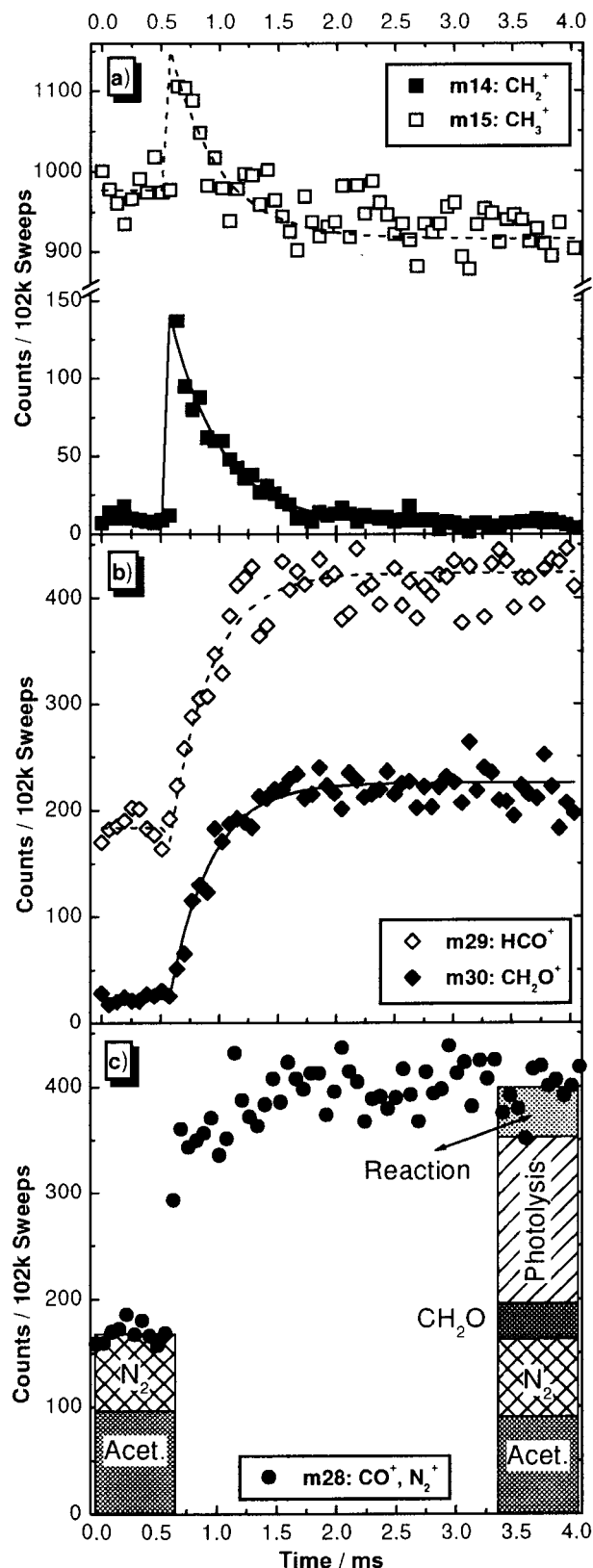
Figure 5. Ion signals of reactants and products plotted vs time recorded in experiment # 5 (see Figure 4 and Table 2). The solid lines in plots (a) and (b) are fits to second-order decay and rise functions. The broken lines were obtained by normalization of the data according to the respective calibration ratios and adjusting for different offsets. Plot (c) shows data for channel m/e = 28 and the contributions to the signal counts from the different sources. First-order rate constants are (a) k' = 2521 \text{ s}^{-1} , (b) k'' = 3220 \text{ s}^{-1} .
