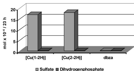
Figure 9. Transport rates of sulfate and dihydrogenphosphate from a mixed \text{SO}_4^{2-}/\text{H}_2\text{PO}_4^- source phase through a \text{CHCl}_3 bulk liquid membrane using the copper complexes [\text{Cu}(\text{L}^1-2\text{H})] , [\text{Cu}(\text{L}^2-2\text{H})] and dibenzylamine (dbza) as carrier. [The concentration of dibenzylamine was 2 mM in the membrane-transport experiments, so that the results could be fairly compared to the dibasic ligands.]
