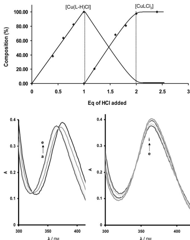
Figure 7. Plot of the formation of the 1:1 and 1:2 [\text{Cu}(\text{L}^2-2\text{H})]/\text{HCl} species in isopropanol at 20°C. The % composition was calculated from the absorbances recorded at the peak formed at 365 nm in the absorption spectra of [\text{Cu}(\text{L}^2-2\text{H})] upon the addition of HCl in isopropanol; the number of equivalents of HCl added are: a) 0, b) 0.4, c) 0.6, d) 0.8, e) 1.0, f) 1.2, g) 1.6, h) 1.8, i) 2.0.
