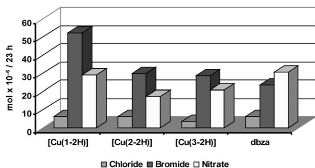
Figure 8. The transport rates of \text{Cl}^- , \text{Br}^- , and \text{NO}_3^- from a mixed anion source phase using [\text{Cu}(\text{L}-2\text{H})] ( \text{L} = \text{L}^1\text{--}\text{L}^3 ) and dibenzylamine (dbza) as carrier. [The concentration of dibenzylamine was 2 mM in the membrane-transport experiments, so that the results could be fairly compared to the dibasic ligands.]
