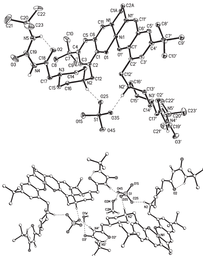
Figure 11. Top: The structure of [Ni(L^6)SO_4]\cdot 1.75H_2O\cdot 2.25MeOH , showing the atom labelling scheme and intramolecular hydrogen bonding. Minor disorder components for the ethane bridge and one t Bu group, all H atoms except NH and all solvent molecules have been omitted. Displacement ellipsoids are drawn at the 30% probability level. Bottom: Intermolecular hydrogen bonding involving the sulfate anions. General notes: The 1,2-diiminoethane links have an approximately syn conformation with an N-C-C-N torsion angles of 45.41 and 19.55° in the major and minor disorder components. The RMS deviation of the N_2O_2 donors and the Ni^{II} cation from their least-squares mean plane is 0.022 Å.
