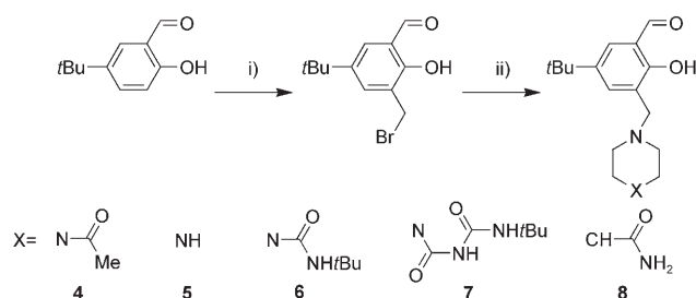
Scheme 3. Synthesis of salicylaldehyde derivative precursors for L^4 – L^7 . i) reference [33]; ii) appropriate piperazine or piperidine, \text{K}_2\text{CO}_3 and \text{KI} in \text{CH}_3\text{CN} . Aldehyde 9 has the same structure as 8 , but with a mixed isomer nonyl group replacing the tert -butyl substituent.
