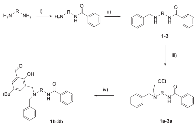
Scheme 2. Synthesis of 1–3 as the secondary amines precursors for the preparation of L^1 – L^3 . i) (\text{PhCO})_2\text{O}/\text{CH}_2\text{Cl}_2 ; ii) \text{PhCHO} , \text{NaBH}_4 ; iii) paraformaldehyde, \text{K}_2\text{CO}_3 , \text{EtOH} , 0^\circ\text{C} , 72 h; iv) 5- tert -butyl-2-hydroxybenzaldehyde, \text{MeCN} , reflux, 72 h.
