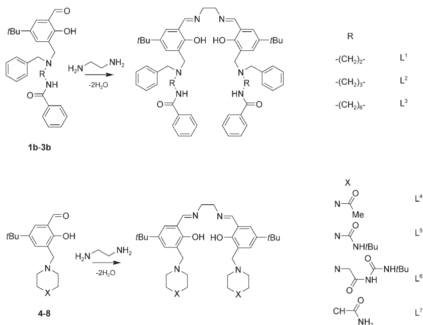
Scheme 1. Preparation of salen derivatives with pendant anion-complexing groups ortho to the phenolate donor atoms. Ligand L^8 has the same structure as L^7 , but with mixed isomer/multibranched nonyl groups replacing the tert -butyl substituents.
