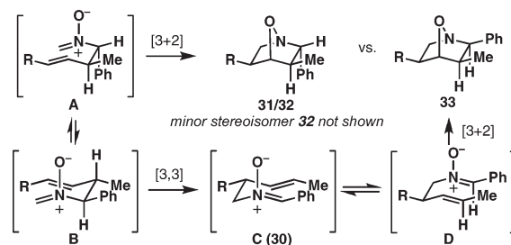
Figure 4. Direct [3 + 2] cycloaddition versus tandem [3,3] rearrangement/[3 + 2] cycloaddition.
