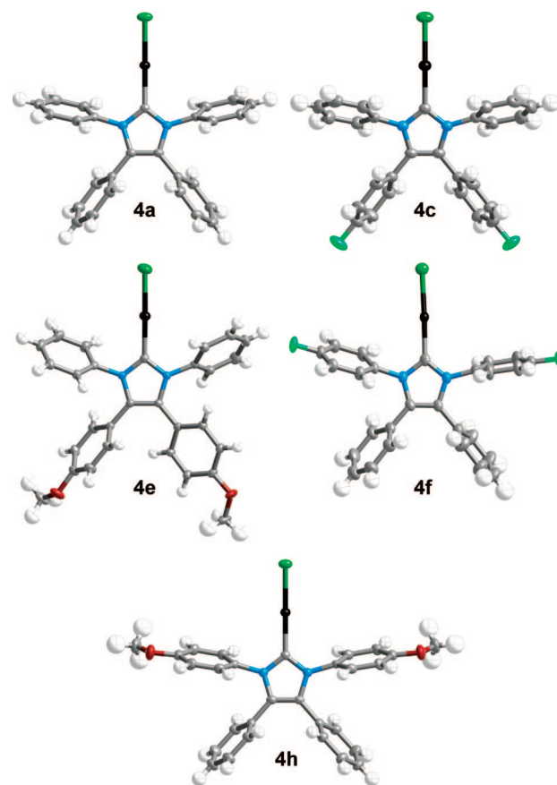
Figure 1. Silver carbene complexes 4a , 4c , 4e , 4f , and 4h depicted with 50% probability ellipsoids.
