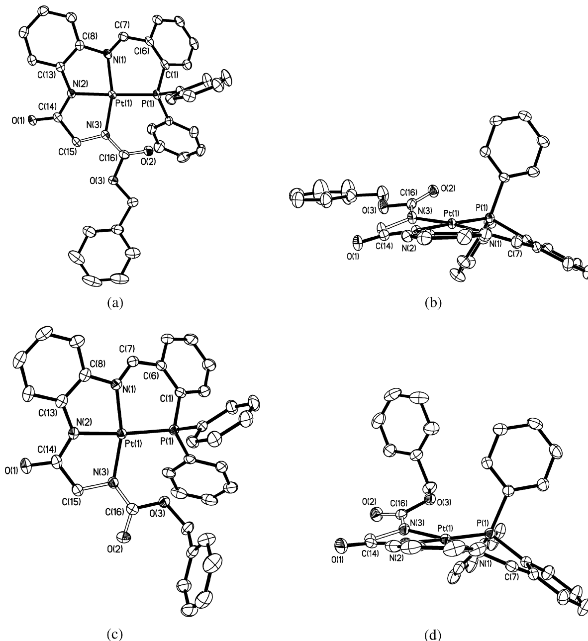
Figure 5. (a) ORTEP plot of \kappa^4 -PNN'N''-tetradentate anti- 6a . (b) Side projection of anti- 6a showing the orientation of the N-C(O)OBz group and the metallocycle ring conformations. (c) ORTEP plot of \kappa^4 -PNN'N''-tetradentate syn- 6a' . (d) Side projection of syn- 6a' showing the orientation of the N-C(O)OBz group and the metallocycle ring conformations. All thermal ellipsoids are drawn at the 50% probability level.
