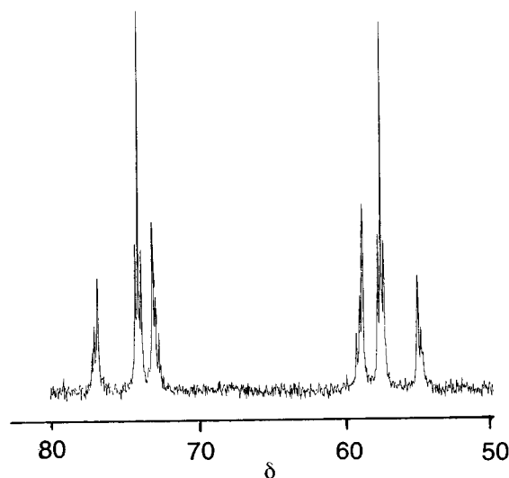
Fig. 1 The ^{31}P\{-^1H\} NMR spectrum (101 MHz, CD_3CN ) of complex 10 , showing the mixture of the two isomers referred to in the text. The two 'virtual' triplets are due to the trans isomer
