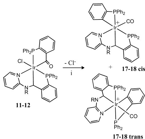
Scheme 4 a
