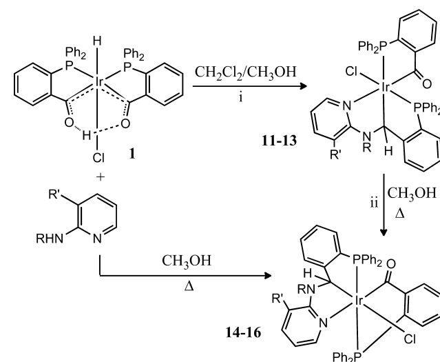
Scheme 3 a
