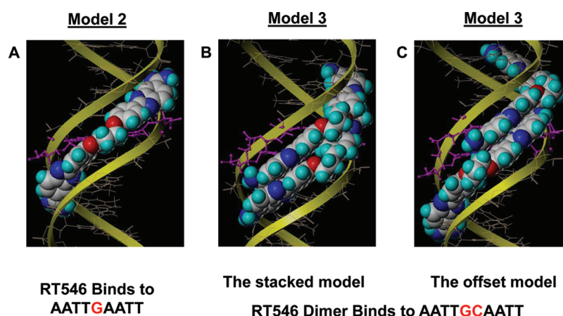
Figure 5. Models for RT546 docked into the (A) AATTGAATT site, Model 2 in Figure 6; and (B and C) the AATTGCAATT sequence (see Model 3 in Figure 6). The complex in (B) is highly overlapped while in (C) the complex is offset. For clarity, the terminal bases are not displayed in the images, and the images are of only the lowest-energy conformation. The DNA backbone is shown by yellow ribbons and the GC base pairs are displayed by ball and stick type in magenta, while the ligand is displayed as spacefill type in CPK colors. More detailed modeling Figures of the models are in Supporting Information, Figure S6.
