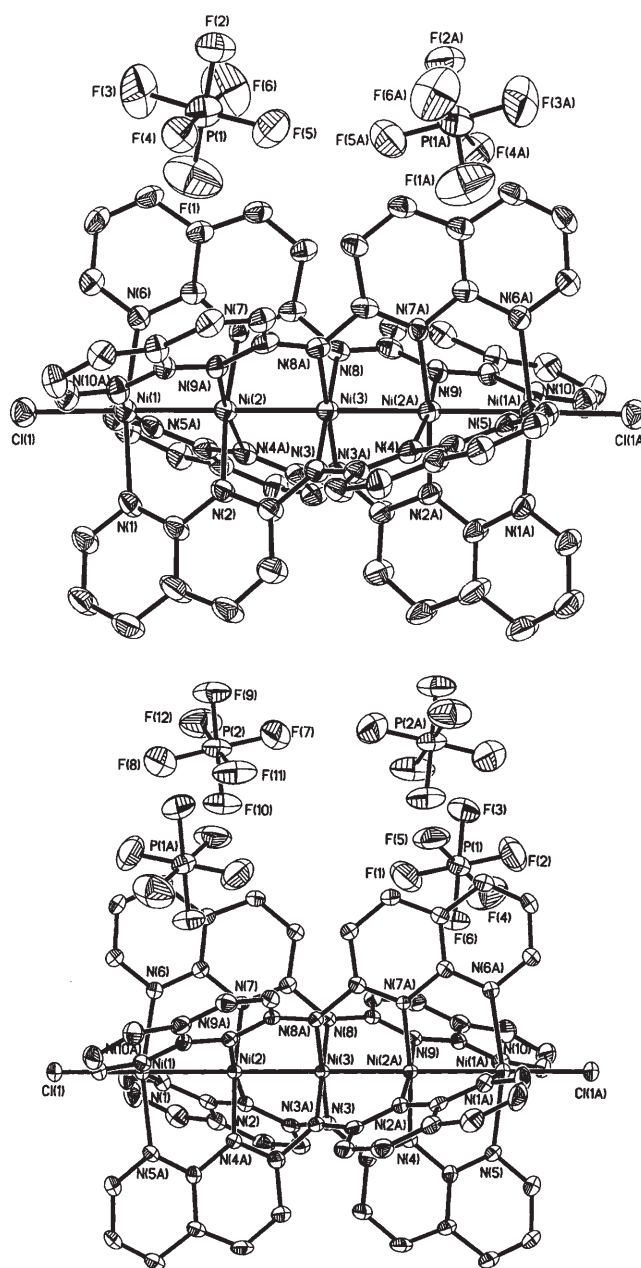
Figure 1. Molecular structures of complexes 1 (top) and 2 (bottom). Ellipsoids are drawn at 30% (top) and at 50% (bottom) probability levels. Hydrogen atoms and interstitial solvents have been omitted for clarity.
