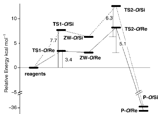
Figure 1. Energy profiles for the outward/Re and outward/Si paths.
