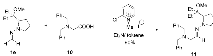
Scheme 4. Reaction between hydrazone 1e and dibenzylglycine 10 .
