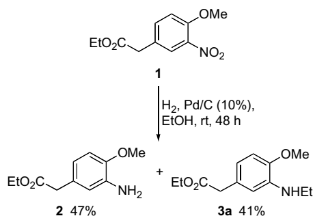
Scheme 1. Initial finding.
