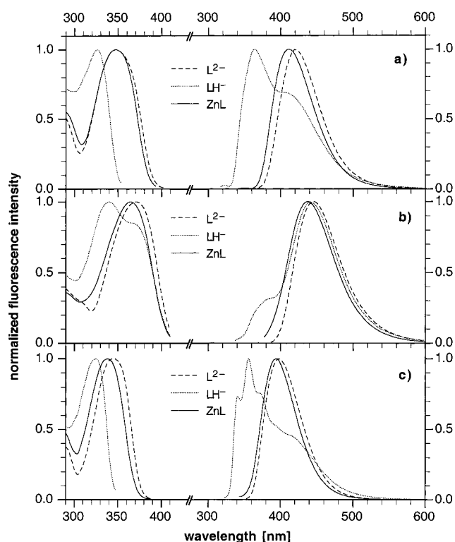
Figure 3. Normalized fluorescence emission and excitation spectra for a) oxazole 4b , b) thiazole 6b and c) imidazole 5b in aqueous solution. All spectra were monitored with 0.1 \text{ M KNO}_3 ionic background at 25^\circ\text{C} . The traces for the monoprotonated ligand ( \text{LH}^- ) were measured at pH 7.20 (10 mM PIPES), the spectra of the fully deprotonated ligand ( \text{L}^{2-} ) were acquired at pH 11.2 (unbuffered). The spectra of the Zn(II) complex were recorded at 5 mM total Zn( \text{OTf} ) 2 for (a) and (c) and 500 mM Zn( \text{OTf} ) 2 for graph (b).
