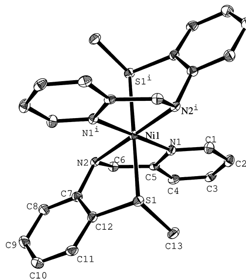
Figure 2. Thermal ellipsoid (probability level 50%) plot of [\text{Ni}(\text{L}2)_2]^{2+} (cation 6) with the atom labeling scheme. H atoms are omitted for the sake of clarity.
