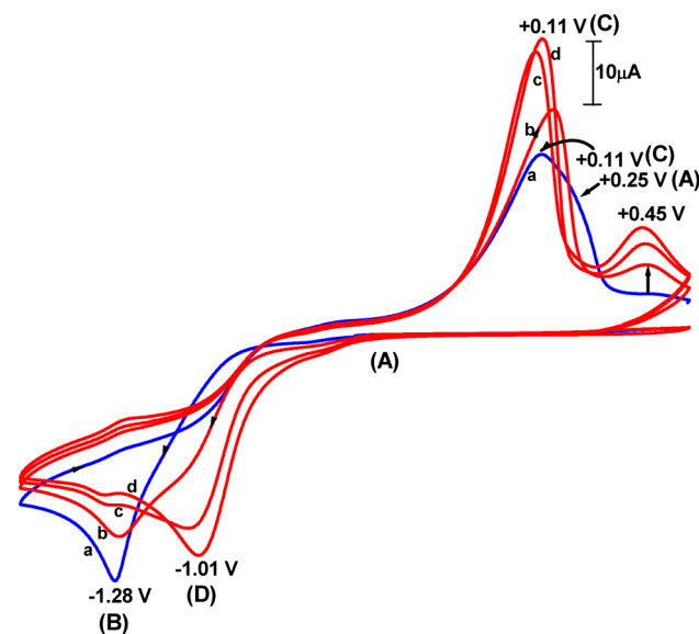
Figure 8. Cyclic voltammograms (a \rightarrow d, repetitive scans) of 6 in \text{CH}_3\text{CN} containing 0.1 \text{ M N}(\text{n-Bu})_4\text{ClO}_4 as supporting electrolyte at 298 \text{ K} at a platinum working electrode at a scan rate 50 \text{ mV s}^{-1} using SCE as reference electrode, showing first scan (a: blue trace) and transformation to [(\text{L2})_2\text{Ni}(\text{CH}_3\text{CN})_2](\text{ClO}_4)_2 (b, c, d: red traces).
