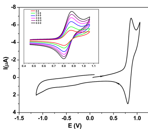
Figure 9. Cyclic voltammograms (scan rate 50 mV/s) of 7 in \text{CH}_3\text{CN} containing 0.1 M \text{N}(\text{n-Bu})_4\text{ClO}_4 as supporting electrolyte at 298 K at a platinum working electrode at a scan rate 50 \text{mV s}^{-1} using SCE as reference electrode.
