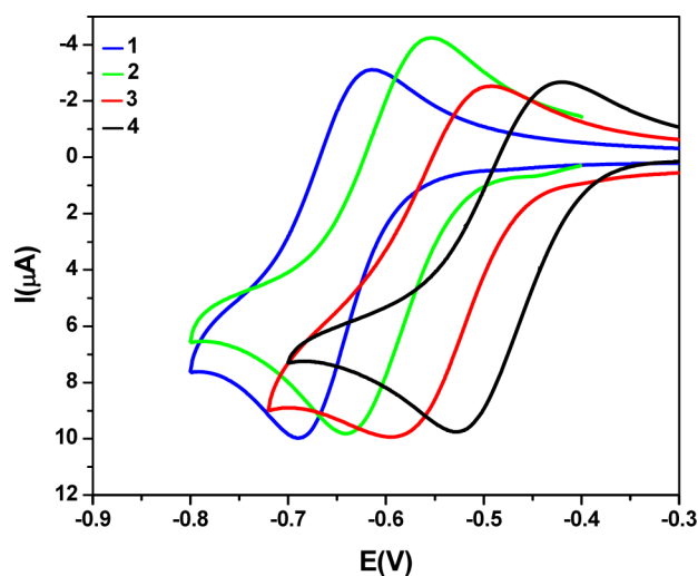
Figure 5. Cyclic voltammograms of 1 (blue), 2 (green), 3 (red), and 4 (black) in CH 3 CN containing 0.1 M n -Bu 4 NClO 4 as a supporting electrolyte at 298 K at a platinum working electrode at a scan rate 50 mV s −1 using SCE as reference electrode.
