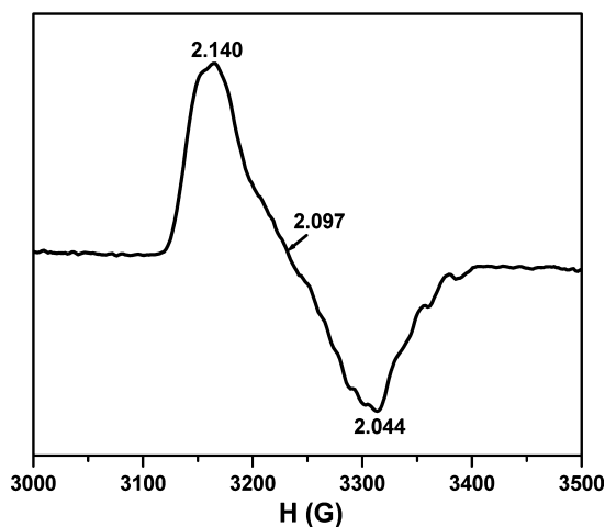
Figure 11. X-band EPR spectrum of electrochemically generated \text{Ni}^{\text{III}} species (from electrolysis of a \text{CH}_3\text{CN} solution of 7 ) at 77 K (conditions: frequency, 9.475 GHz; modulation, 5G; power, 0.189 mW).
