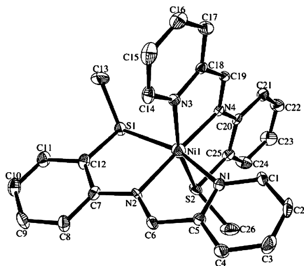
Figure 1. Thermal ellipsoid (probability level 50%) plot of [\text{Ni}(\text{L}1)_2]^{2+} (cation 1) with the atom labeling scheme. H atoms are omitted for the sake of clarity.
