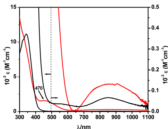
Figure 10. Electronic absorption spectra of 7 (black) and of the coulometrically generated oxidized species [(\text{L}3)_2\text{Ni}^{\text{III}}]^+ (red) containing 0.1 M \text{N}(\text{n-Bu})_4\text{ClO}_4 at 298 K. The arrow indicates the Y-scale of the peaks from dashed line.
