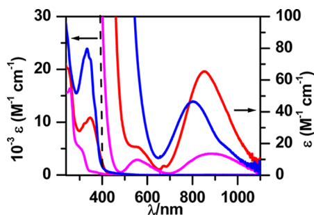
Figure 4. Electronic absorption spectra of [Ni(L1)_2](ClO_4)_2 , 1 (blue), [Ni(L2)_2](ClO_4)_2 , 6 (pink), and [Ni(L3)_2] , 7 (orange) in CH_3CN .
