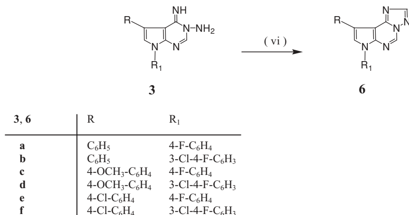
SCHEME 2 Reagent and conditions (vi) CH(OC 2 H 5 ) 3 or HCOOH, Reflux, 5–6 h.
