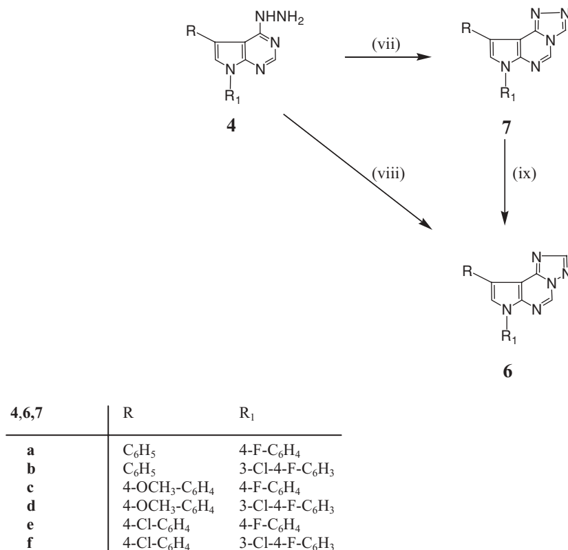
SCHEME 3 Reagent and conditions (vii) CH(OC 2 H 5 ) 3 , 70°C, 1–1.5 h.; (viii) HCOOH, Reflux, 6–8 h.; (ix) HCOOH, reflux, 3–4 h.
