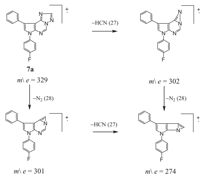
SCHEME 4 Mass fragmentation pattern of 7a .
