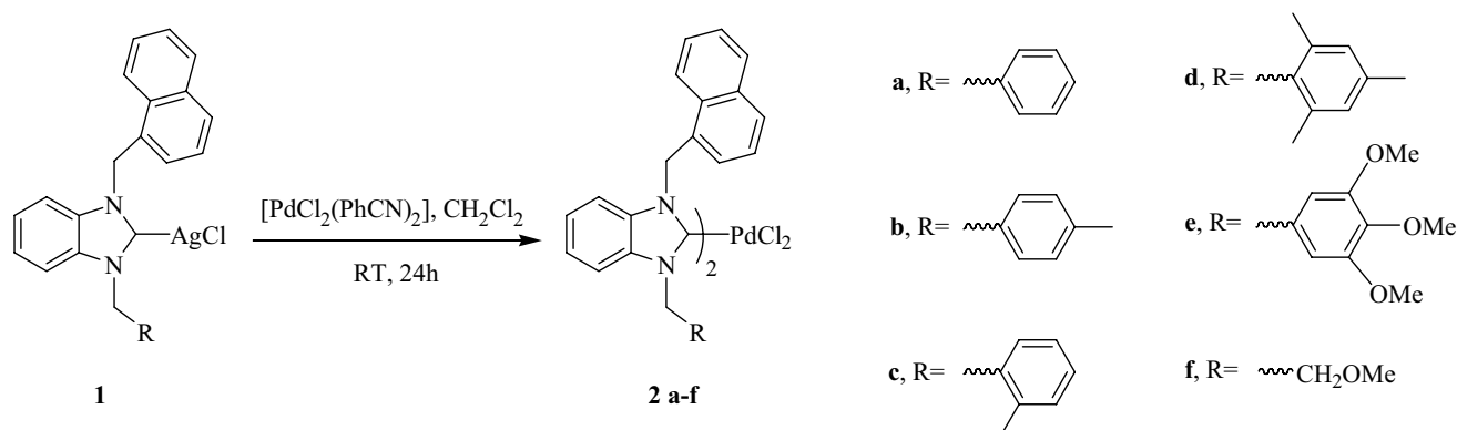
Scheme 1 Synthesis of the palladium(II) NHC complexes
