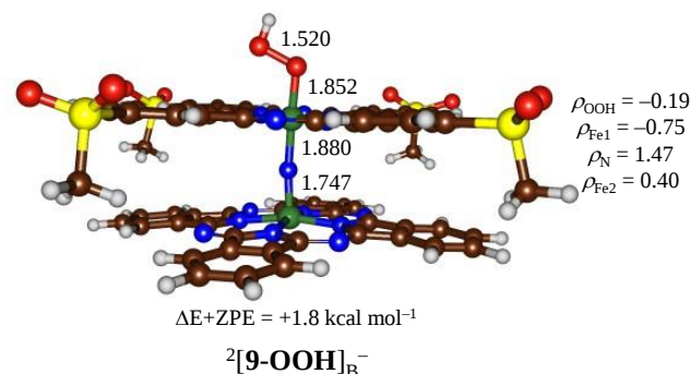
Fig. 7. DFT optimized geometries of 2[\mathbf{9}\text{-OOH}] at the B3LYP level of theory. Bond lengths are in angstroms and spin densities ( \rho ) in atomic units.
