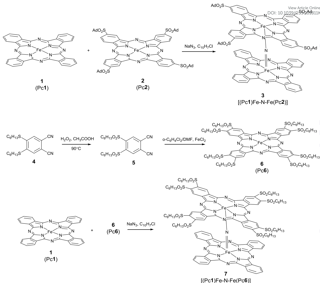
Scheme 2. Preparation of heteroleptic \mu -nitrido alkylsulfonyl phthalocyaninato iron(II) 3 and 7 .
