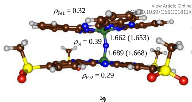
Fig. 6. DFT optimized geometries of \mathbf{9} at the B3LYP (BP86) level of theory. Bond lengths are in angstroms and spin densities ( \rho ) in atomic units.
