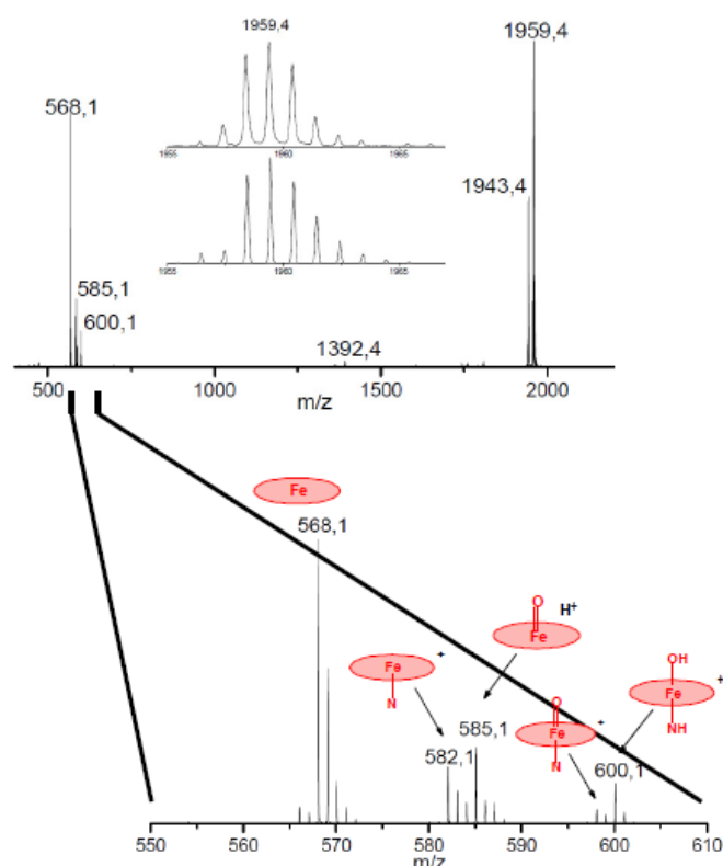
Fig 4. CID MS/MS spectrum of the oxo complex ( 3=O ) obtained from 3 and \text{H}_2\text{O}_2 . Inset: comparison of experimental (top) and simulated (bottom) isotopic distribution of molecular peak. An enlarged region of spectrum with assignment of fragments is shown below.
