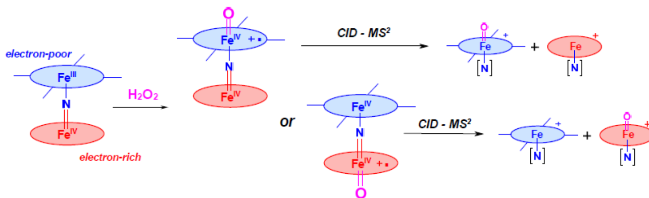
Scheme 3. Formation of isomeric iron(IV)-oxo complexes with heteroleptic ligands and schematic representation of its fragmentation patterns. Blue ligand: substituted with SO_2R groups. Red ligand: unsubstituted phthalocyanine.
