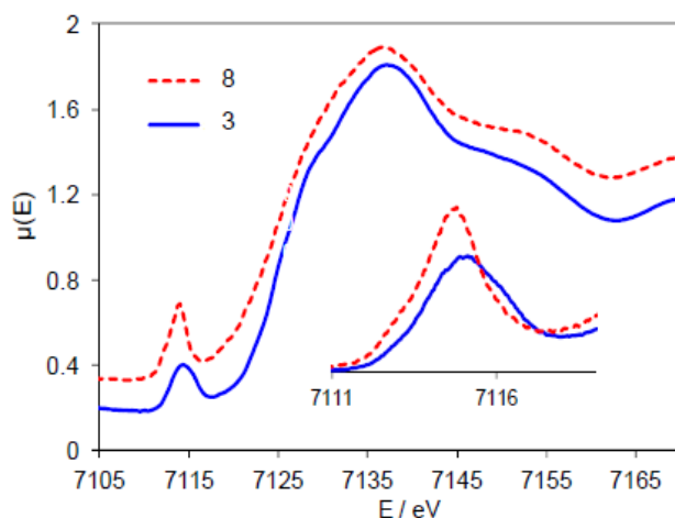
Fig 2. Experimental XANES spectra of heteroleptic complex 3 and homoleptic complex 8 . Inset – superposition of their pre-edge regions.
