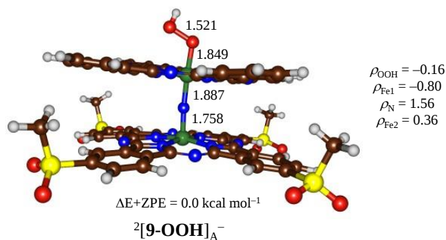
Fig. 6. DFT optimized geometries of \mathbf{9} at the B3LYP (BP86) level of theory. Bond lengths are in angstroms and spin densities ( \rho ) in atomic units.
