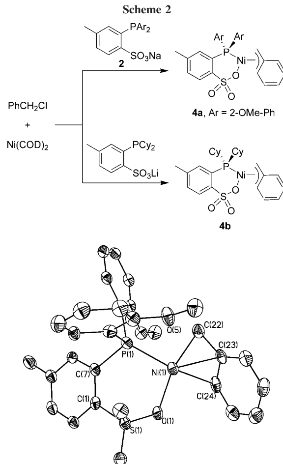
Figure 1. Molecular structure of 4a . Hydrogen atoms are omitted. Selected bond distances (Å) and angles (deg): Ni(1)–P(1) 2.163(1), Ni(1)–O(1) 1.938(3), Ni(1)–C(22) 1.949(4), Ni(1)–C(23) 2.066(4), Ni(1)–C(24) 2.191(4), S(1)–O(1) 1.499(3), S(1)–O(2) 1.443(3), S(1)–O(3) 1.446(3); O(1)–Ni(1)–P(1) 99.34(8), P(1)–Ni(1)–C(22) 96.8(1), O(1)–Ni(1)–C(24) 91.7(1), C(22)–Ni(1)–C(24) 71.8(2).
