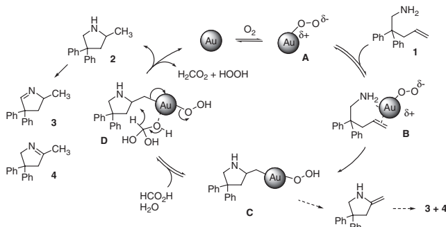
Scheme 1. Proposed mechanism.
