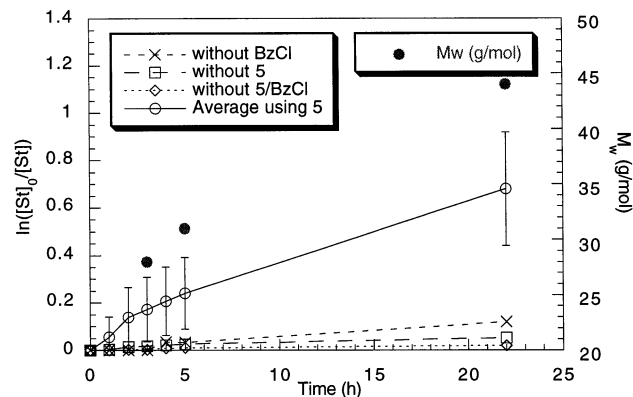
Fig. 4. Semilogarithmic plot of styrene conversion vs. time. (i) Without BzCl, (ii) without molybdenum compound ( 5 ), (iii) without BzCl nor 5 , and (iv) average in the presence of BzCl and 5 .
