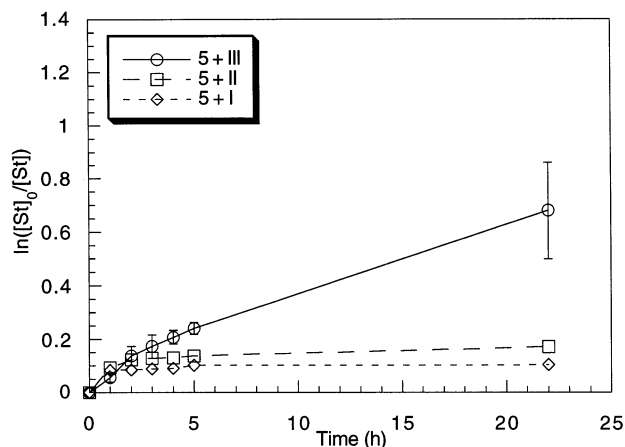
Fig. 3. Semilogarithmic plot of styrene conversion vs. time using different initiators ( [\text{St}]_0 = 3 \text{ M} , [\textbf{5}] = 0.03 \text{ M} , [\text{XC(Ph)HR}]_0 = 0.03 \text{ M} in toluene at 80°C).
