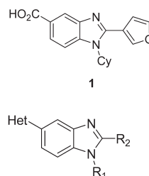
Figure 1. Candidates for an allosteric inhibitor of hepatitis C virus (HCV) NSSB polymerase.
