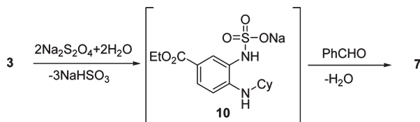
Scheme 3. Plausible mechanism of the reductive cyclization
