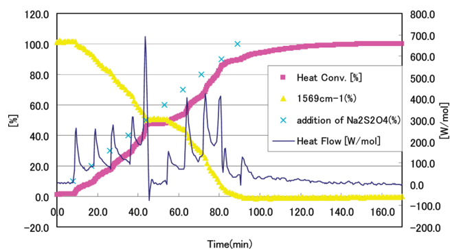
Figure 5. Heat flow of the semibatch-type operation of the reaction in \text{DMSO}/\text{H}_2\text{O} .
