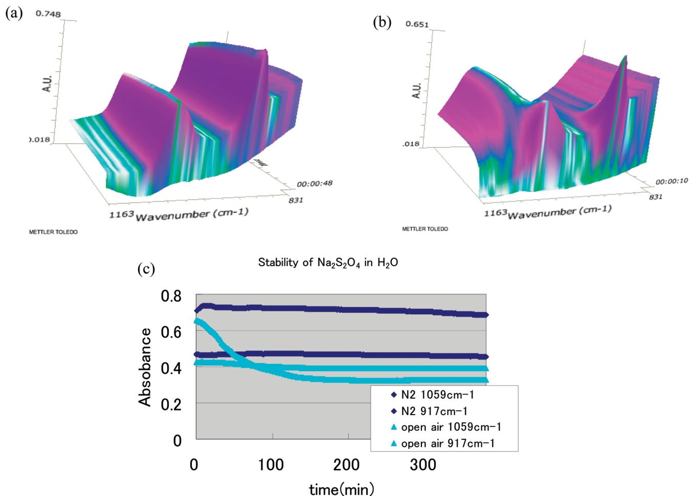
Figure 4. (a) Stability of \text{Na}_2\text{S}_2\text{O}_4 in \text{H}_2\text{O} (20 wt %) in nitrogen atmosphere. (b) Stability of \text{Na}_2\text{S}_2\text{O}_4 in \text{H}_2\text{O} (20 wt %) in air atmosphere, (c) Change of absorbance of in situ IR analysis.
