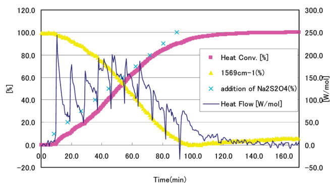
Figure 6. Heat flow of the semibatch-type operation of the reaction in \text{DMA}/\text{H}_2\text{O} .
