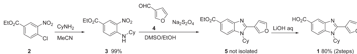
Scheme 2. Synthesis of 1 using reductive cyclization
