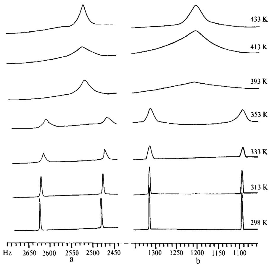
Figure 2. Temperature dependent ^1\text{H} NMR spectra of 7a in \text{DMSO}-d_6 : a- region of H-2 signal; b - region of N-methyl group.
