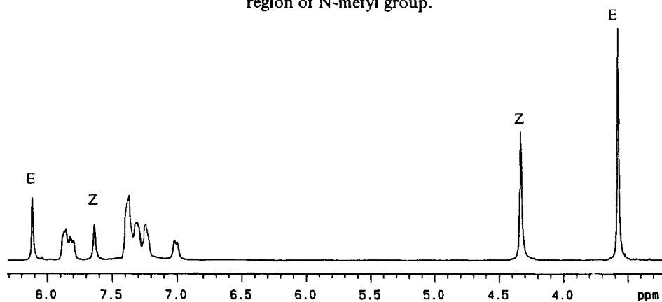
Figure 3. ^1\text{H} NMR spectrum of 7a in \text{CDCl}_3 .
