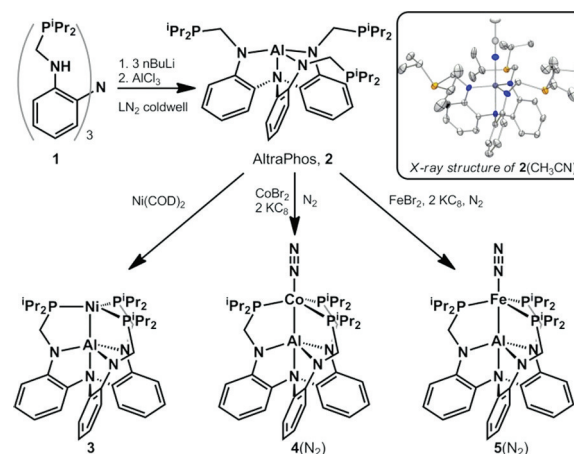
Scheme 1. Syntheses of Proligand 1 , AltraPhos ( 2 ) and the Metallalumatrane Coordination Complexes and Structure of 2
