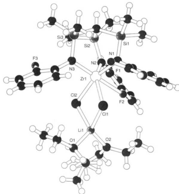
Figure 6. Molecular structure of \text{HC}\{\text{SiMe}_2\text{N}(2\text{-FC}_6\text{H}_4)\}_3\text{ZrCl}_2\text{Li}(\text{OEt}_2)_2 ( 4 ) in the crystal.
