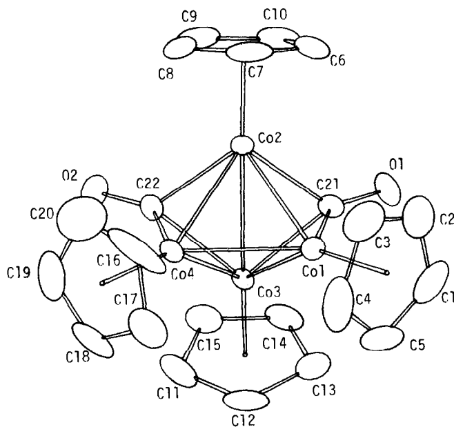
Fig. 1. Molecular structure of complex III, [\text{Cp}_4\text{Co}_4(\mu_3\text{-CO})_2] . Bond distances (Å): Co(1)—Co(2), 2.381(2); Co(1)—Co(3), 2.397(2); Co(1)—Co(4), 2.395(2); Co(2)—Co(3), 2.455(2); Co(2)—Co(4), 2.409(2); Co(3)—Co(4), 2.399(2); Co(1)—C(21), 1.890(8); Co(2)—C(21), 1.946(8); Co(2)—C(22), 1.970(8); Co(3)—C(21), 1.952(8); Co(3)—C(22), 1.987(8); Co(4)—C(22), 1.890(8); Co(1)—Cp(1), 1.73(2); Co(2)—Cp(2), 1.72(1); Co(3)—Cp(3), 1.73(1); Co(4)—Cp(4), 1.73(2); C(21)—O(1), 1.21(1); C(22)—O(2), 1.20(1).
