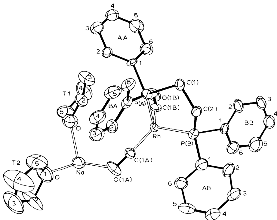
Fig. 2. A perspective view of [\text{Na}(\text{THF})_2][\text{Rh}(\text{CO})_2(\text{Diphos})] . Principle bond lengths ( \text{\AA} ): \text{Rh}-\text{C}(1\text{A}) , 1.84; \text{Rh}-\text{C}(1\text{B}) , 1.850; \text{Rh}-\text{P}(\text{A}) , 2.306; \text{Rh}-\text{P}(\text{B}) , 2.300; \text{C}(1\text{A})-\text{O}(1\text{A}) , 1.158; \text{C}(1\text{B})-\text{O}(1\text{B}) , 1.181; \text{Na}-\text{O}(1\text{A}) , 2.408; \text{Na}-\text{O}(\text{1T1}) 2.303; \text{Na}-\text{O}(\text{1T2}) , 2.283. Principle bond angles (degrees): \text{C}(1\text{A})-\text{Rh}-\text{C}(1\text{B}) , 116.6; \text{C}(1\text{A})-\text{Rh}-\text{P}(\text{A}) , 113.1; \text{C}1\text{A}-\text{Rh}-\text{P}(\text{B}) , 117.1; \text{C}(1\text{B})-\text{Rh}-\text{P}(\text{A}) , 102.6; \text{C}(1\text{B})-\text{Rh}-\text{P}(\text{B}) , 116.2; \text{P}(\text{A})-\text{Rh}-\text{P}(\text{B}) , 85.76; \text{Rh}-\text{C}(1\text{A})-\text{O}(1\text{A}) , 174.8; \text{Rh}-\text{C}1\text{B}-\text{O}1\text{B} , 171.6; \text{C}(1\text{A})-\text{O}(1\text{A})-\text{Na} , 121.2; \text{O}(1\text{A})-\text{Na}-\text{O}(\text{1T1}) , 106.8; \text{O}(1\text{A})-\text{Na}-\text{O}(\text{1T2}) , 98.1; \text{O}(\text{1T1})-\text{Na}-\text{O}(\text{1T2}) , 98.8.
