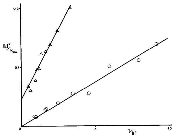
Figure 3. Plots of [L]^2/k_{\text{obs}} vs. 1/[L] (eq. 8) at 24.8 °C: \Delta BZA; \circ CHA.
