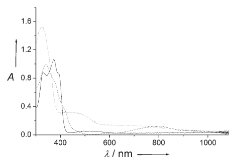
Figure 6. Electronic spectra of 0.05 mM solutions of [\text{Ni}(\text{L}^3)]^{2-} (solid lines) and electrogenerated [\text{Ni}(\text{L}^3)]^- (dashed lines) in \text{CH}_2\text{Cl}_2 (+0.005 M TBAP). The dotted lines represent [\text{Ni}(\text{L}^3)]^- in the presence of 25 mM pyridine. T=233\text{ K} , l=1.000\text{ cm} .
