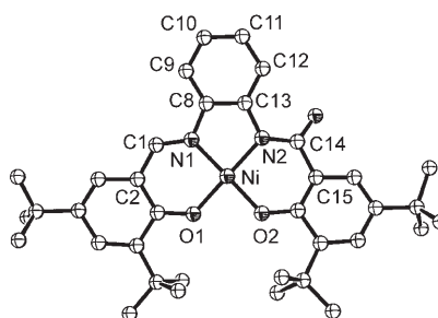
Figure 2. X-ray crystal structure of [\text{Ni}(\text{L}^2)]^- ( 2 ) shown with 30 % thermal ellipsoids.
