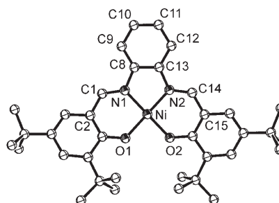
Figure 1. X-ray crystal structure of [\text{Ni}(\text{L}^1)] ( 1 ) shown with 30 % thermal ellipsoids.
