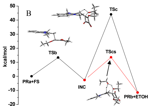
Figure 4. Energy profiles for (A) the deprotonation of benzimidazole salt by base, and (B) the formation of PRb.
