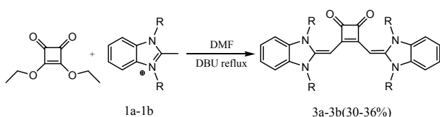
Scheme 3. Reaction of Benzimidazole Salts (1a-b) and 3,4-Diethyl Squarate catalyzed by DBU in dry DMF.
