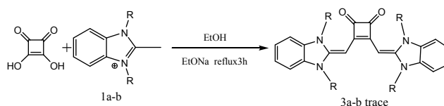
Scheme S2. The reaction between benzimidazole salt and squaric acid catalyzed by EtONa.
