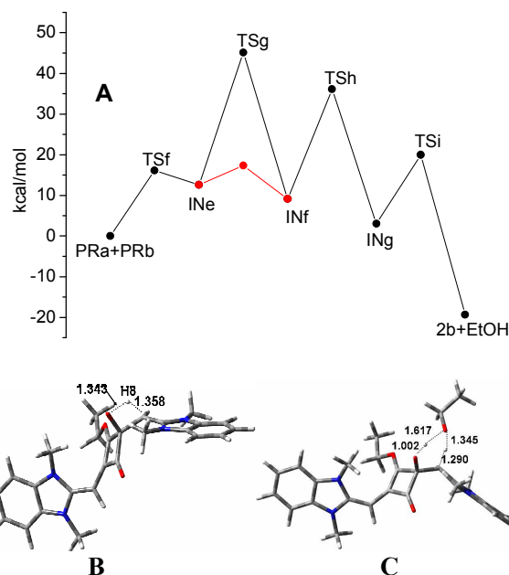
Figure 6. Energy profiles for the formation of 2b (pathways: I-B) and the structures of transition states (B: TSg, C: TSi).
