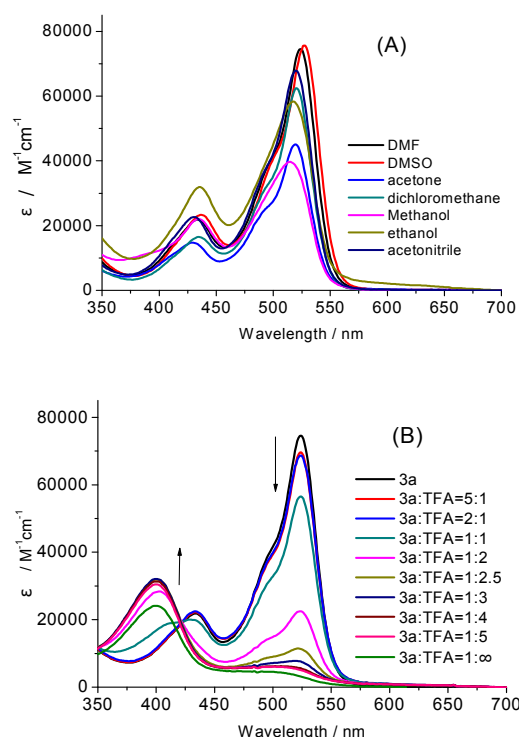
Figure 2. Absorption spectra of the 1,2-SQ 3a in various solvents (A). Absorption spectra change of 3a in acetone upon addition of different ratio of trifluoroacetic acid (TFA) (B).
