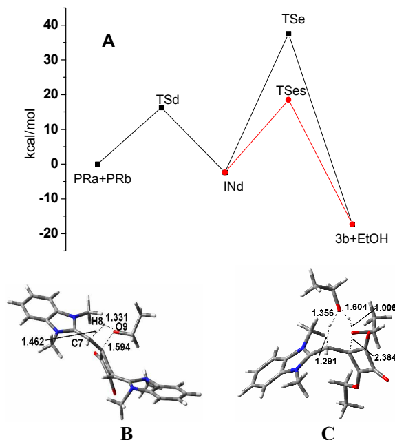
Figure 5. Energy profiles for the formation of 3b (pathways: I-A) and the structures of transition states (B: TSd, C: TSe).
