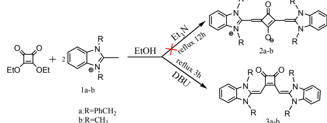
Scheme 1. The reaction of benzimidazole salt with 3,4-diethyl squarate.
