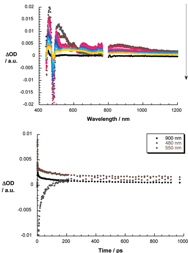
Figure 4. (Top) Differential absorption spectra (visible and near-infrared) obtained upon femtosecond flash photolysis (387 nm, 150 nJ) of Mn(III)Cl-2 ( \sim 10^{-6} M) in argon saturated PhCN with several time delays between 0 and 3 ns at room temperature; see legend for time evolution. (Bottom) time absorption profiles at 480, 550, and 900 nm of the spectra shown above, monitoring the charge separation and charge recombination.
