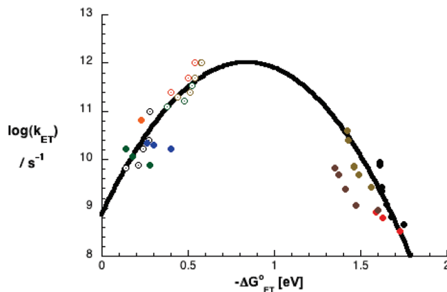
Figure 8. Driving force ( -\Delta G^0_{ET} ) dependence of the rate constant for charge separation (open circles) and charge recombination (full circles) in Mn(III)Cl-1 , Mn(III)Cl-2 (blue symbols), Fe(III)Cl-1 , Fe(III)Cl-2 (orange symbols), Co(II)-3 (grey symbols), 30 Ni(II)-1 , Ni(II)-2 (green symbols), Cu(II)-1 , Cu(II)-2 (red symbols), Zn(II)-1 , Zn(II)-2 (brown symbols), H 2 -1 , and H 2 -2 (black symbols).
