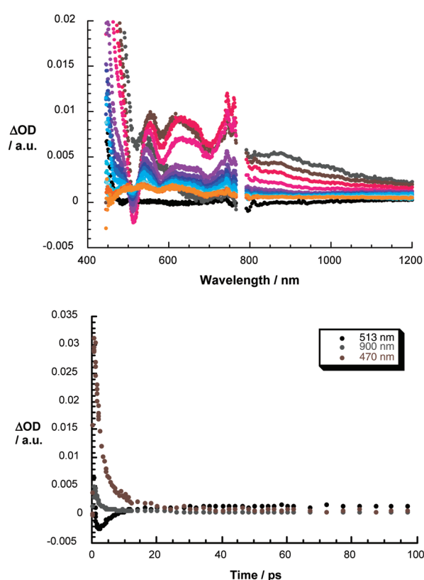
Figure 5. (Top) differential absorption spectra (visible and near-infrared) obtained upon femtosecond flash photolysis (387 nm, 150 nJ) of Fe(III)Cl-2 ( \sim 10^{-6} M) in argon saturated benzonitrile with several time delays between 0 and 50 ps at room temperature; see legend for time evolution. (Bottom) Time absorption profiles at 470, 513, and 900 nm of the spectra shown above, monitoring the charge separation and charge recombination.
