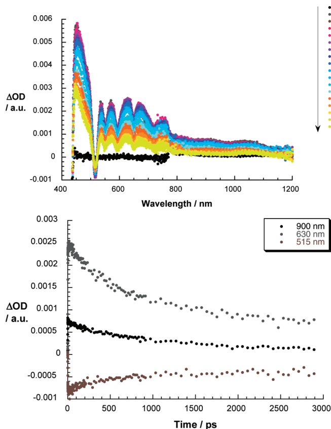
Figure 2. (Top) Differential absorption spectra (visible and near-infrared) obtained upon femtosecond flash photolysis (420 nm, 100 nJ) of H 2 -2 ( \sim 10^{-6} M) in argon saturated THF with several time delays between 0 and 3000 ps at room temperature; see legend for time evolution. (Bottom) Time absorption profiles at 515, 630, and 900 nm of the spectra shown above, monitoring the charge separation and charge recombination.
