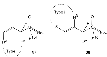
Scheme 9. Definition of Type I and Type II Cycloalkenylsulfoximines
