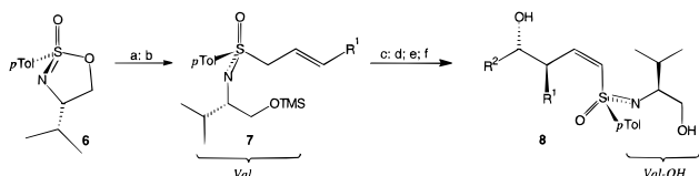
Scheme 3 \gamma -Hydroxyalkylations of Acyclic 2-Alkenylsulfoximines a,b
