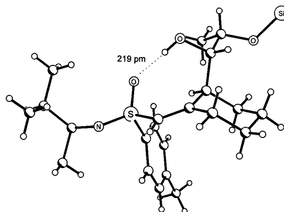
Figure 1. XRAST drawing of a part of the solid state structure of 59 showing the hydrogen bond between the oxygen atom of the sulfoximine moiety and the OH-group at C-4. The double bond between C-1 and C-2 is cis -configured, and the substituent at C-3 in the cyclohexane ring introduced by the aldehyde addition adopts an axial position.
