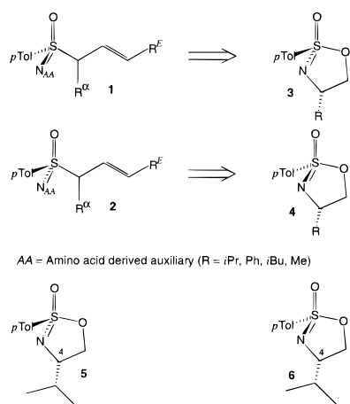
Scheme 3 \gamma -Hydroxyalkylations of Acyclic 2-Alkenylsulfoximines a,b
