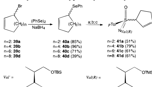
Scheme 10. Synthesis of Type I Cycloalkenylsulfoximines a
