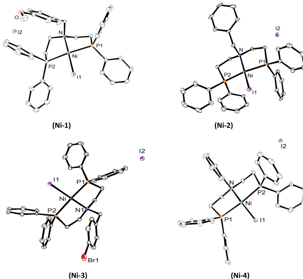
Figure 3. ORTEP diagrams (50% thermal ellipsoids): [(\text{MeO}_{\text{Bz}}\text{NP2})\text{Ni}(\text{I})]\text{I} (Ni-1); [(\text{Bz}\text{NP2})\text{Ni}(\text{I})]\text{I} (Ni-2); [(\text{Br}_{\text{Bz}}\text{NP2})\text{Ni}(\text{I})]\text{I} (Ni-3); [(\text{Ph}\text{NP2})\text{Ni}(\text{I})]\text{I} (Ni-4).
