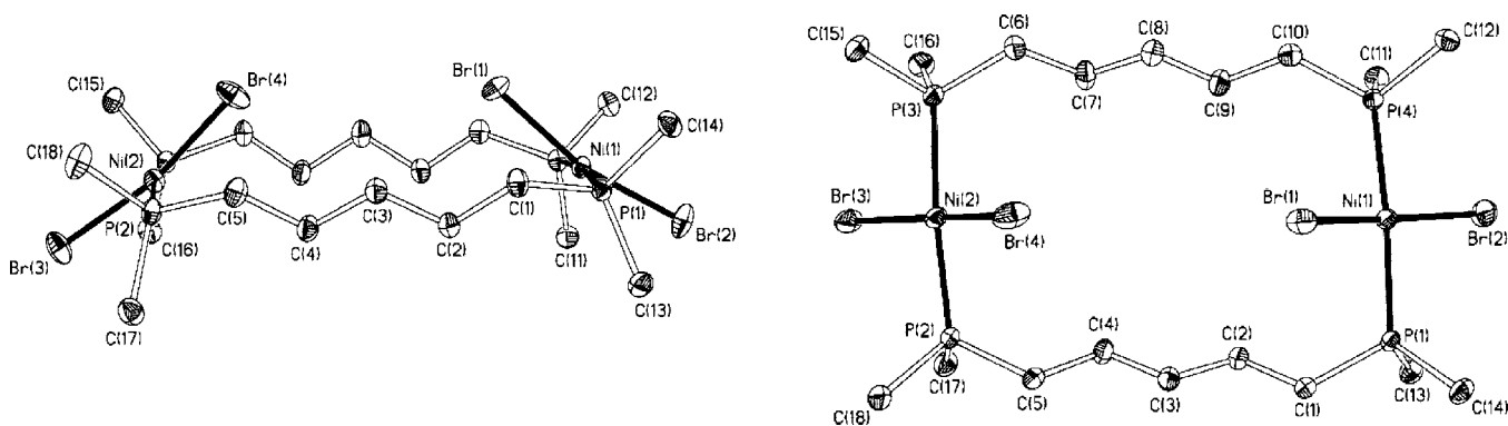
Figure 1. ORTEP diagrams for complex 1 . Thermal ellipsoids are shown at the 30% probability level. Hydrogens and i -Pr methyl carbons are omitted for clarity. Selected bond distances ( \text{\AA} ) and angles (deg): \text{Ni}(1)\text{--P}(1) = 2.2494(10) , \text{Ni}(1)\text{--P}(4) = 2.2466(10) , \text{Ni}(2)\text{--P}(2) = 2.2680(10) , \text{Ni}(2)\text{--P}(3) = 2.2704(10) , \text{Ni}(1)\text{--Br}(1) = 2.3038(6) , \text{Ni}(1)\text{--Br}(2) = 2.3125(7) , \text{Ni}(2)\text{--Br}(3) = 2.3244(7) , \text{Ni}(2)\text{--Br}(4) = 2.3013(7) , \text{P}(1)\text{--Ni}(1)\text{--P}(4) = 171.85(4) , \text{P}(2)\text{--Ni}(2)\text{--P}(3) = 173.36(4) , \text{Br}(1)\text{--Ni}(1)\text{--Br}(2) = 165.99(3) , \text{Br}(3)\text{--Ni}(2)\text{--Br}(4) = 167.83(4) .
