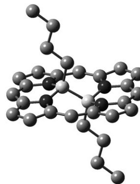
Figure 6. Calculated structure for [( Bn Bu) 2 (porphine)] (B3LYP/6-311-G(d)). Hydrogen atoms have been omitted for clarity.
