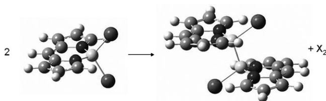
Figure 3. Structures calculated for boryl and diboranyl dipyrromethene (dpm) complexes (B3LYP/6-311G(d,p)).
