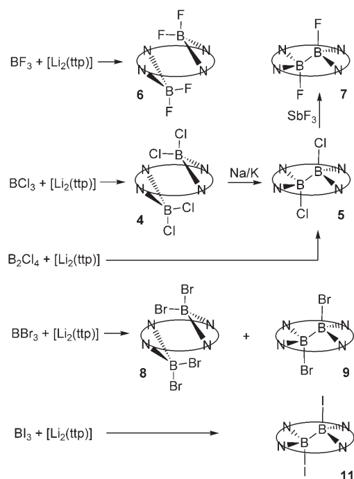
Scheme 1. Synthetic routes for the preparation of [(\text{BX}_2)_2(\text{ttp})] ( \text{X}=\text{F} ( 6a ), \text{Cl} ( 4a ), \text{Br} ( 8a )) and [(\text{BX})_2(\text{ttp})] ( \text{X}=\text{F} ( 7a ), \text{Cl} ( 5a ), \text{Br} ( 9a ), \text{I} ( 11a )).
