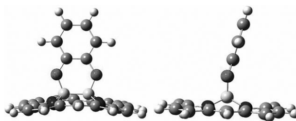
Figure 4. Structure calculated for [\text{B}_2(\text{cat})(\text{porphine})] ( 12 , cat: 1,2- \text{C}_6\text{H}_4\text{O}_2 ) (B3LYP/6-311G(d,p)).
