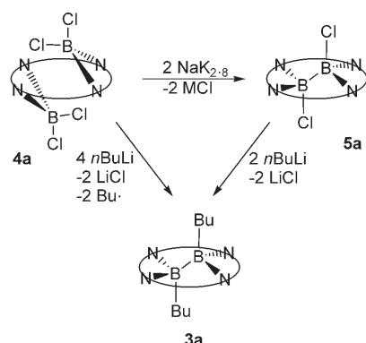
Scheme 4. Reactions of [(BCl 2 ) 2 (tp)] ( 4a ) and [(BCl 2 ) 2 (tp)] ( 5a ) with n BuLi.
