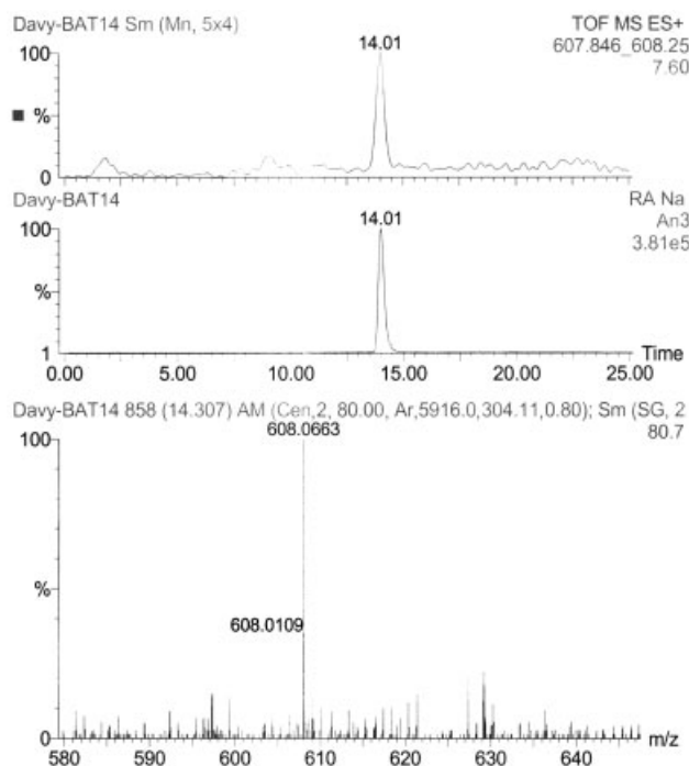
Figure 2. Radio-LC-MS analysis of Tc-techmazenil (A) Single mass chromatogram (607.846–608.250): peak with R_t : 14.01'. (B) Radiometric channel: peak with identical R_t as peak in A. (C) Experimental mass spectrum (relative error: 7.4 ppm)
