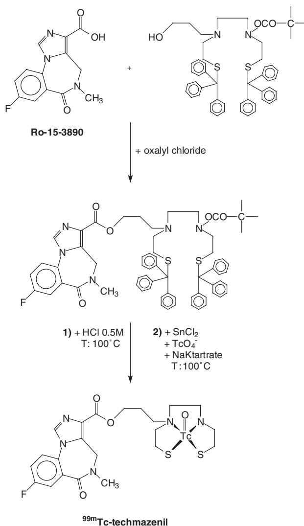
Figure 1. Synthesis of bis-S-trityl-N-Boc-N'-(3-propyl)-BAT ester of Ro-15-3890 and ^{99m}\text{Tc} -techmazetil (proposed structure)
