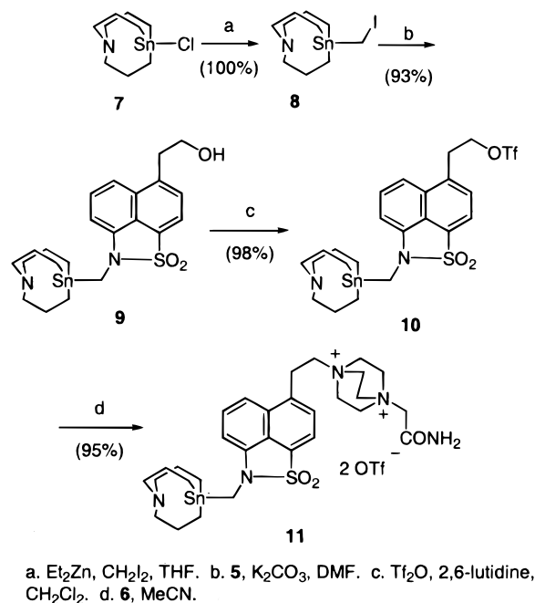
Scheme 2. Preparation of the Stannatrane Coupling Partner
