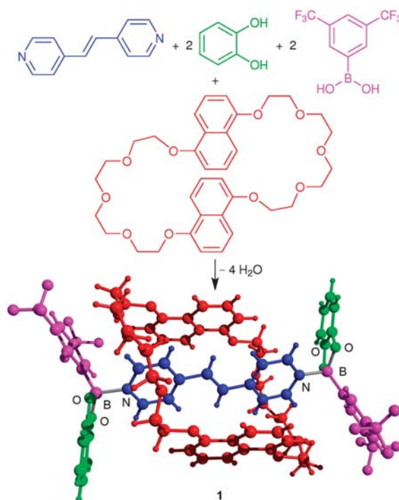
Scheme 1 Synthesis of rotaxane 1 . The graphic representation of 1 is based on a crystallographic analysis.
