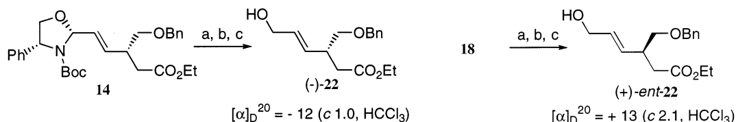
Scheme 5. Reagents and conditions: (a) \text{CF}_3\text{COOH} , DCE. (b) \text{THF} , \text{H}_2\text{O} . (c) \text{NaBH}_4 , \text{CeCl}_3 , 7\text{H}_2\text{O} , \text{EtOH} , 0^\circ\text{C} . 22 : 72%; ent - 22 : 52%
