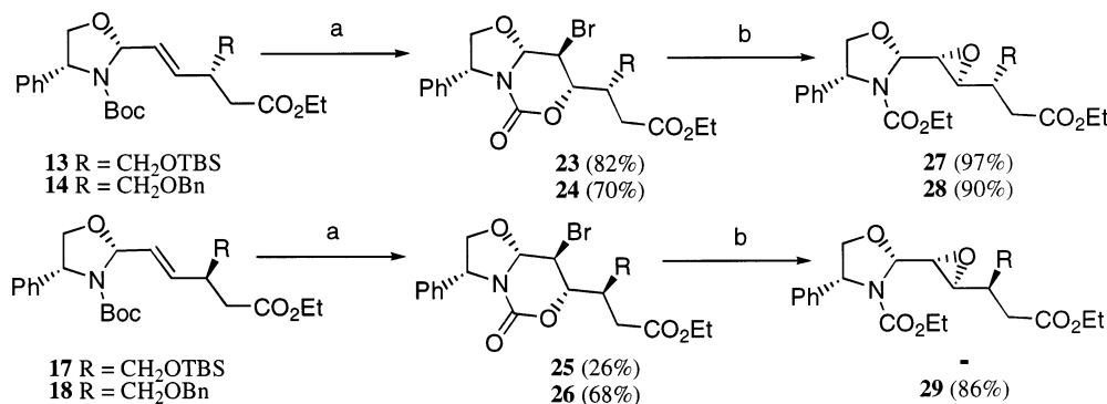
Scheme 6. Reagents and conditions: (a) \text{NBS} , \text{DME}/\text{H}_2\text{O} . (b) \text{EtONa}/\text{EtOH}
