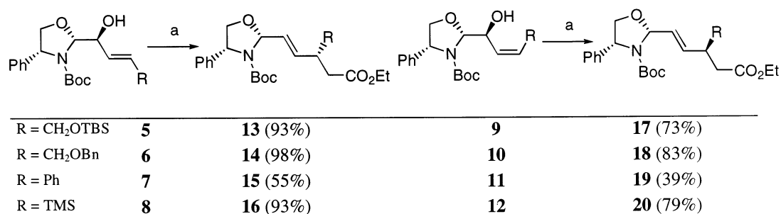
Scheme 3. Reagents and conditions: (a) \text{CH}_3\text{C}(\text{OEt})_3 , propionic acid (cat.), reflux, 3 h 6d
