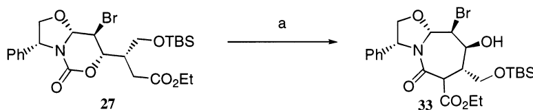
Scheme 9. Reagents and conditions: (a) LiHMDS, THF, –50°C, 61%
