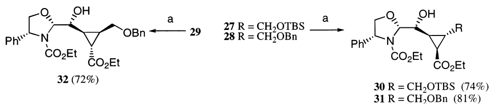
Scheme 7. Reagents and conditions: (a) LiHMDS, THF, –50°C
