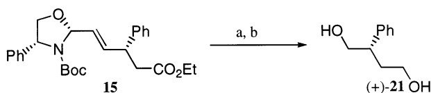
Scheme 4. Reagents and conditions: (a) \text{OsO}_4 (cat.), \text{NaIO}_4 , \text{THF}/\text{H}_2\text{O} . (b) \text{NaBH}_4 , \text{EtOH} , 53% overall yield
