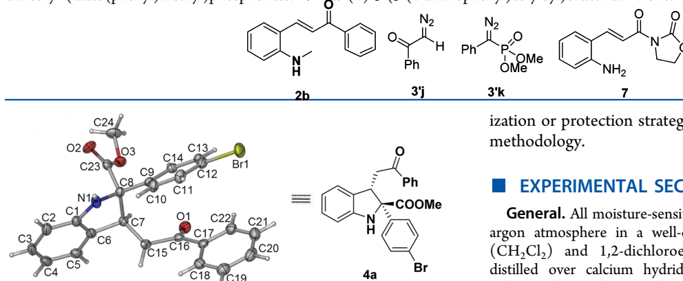
Figure 2. Single-crystal X-ray of 4a.
