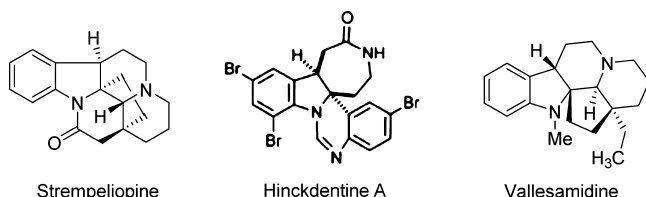
Figure 1. Examples of biologically active 2,3-multisubstituted indolines.
